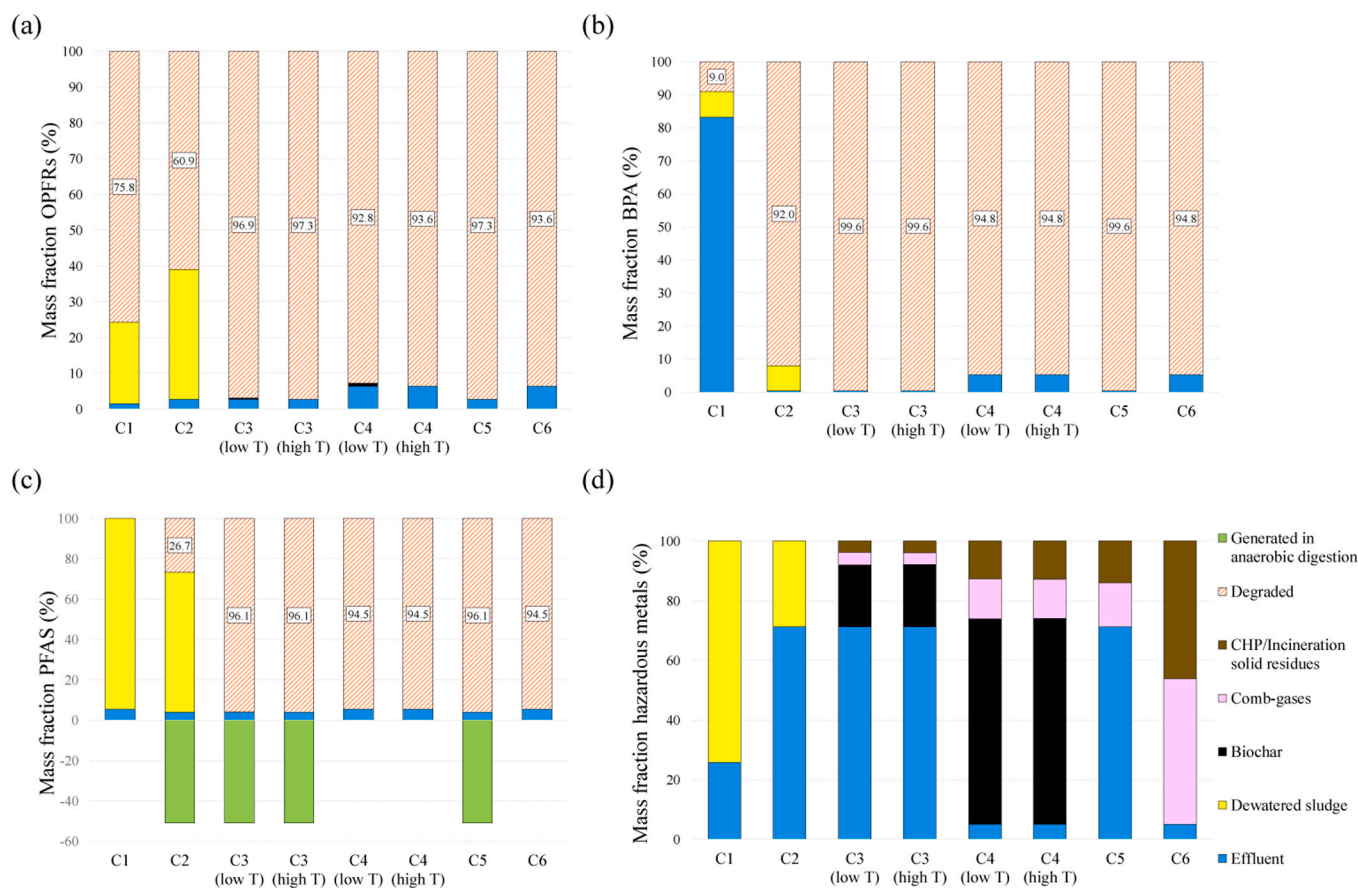
Fig. 3. Mass fraction (%) relative to total initial loading (100%) in the raw sewage sludge showing the percentage of degradation and fate of OPFRs (a), BPA (b), PFAs (c) and HMs (d). Effluent indicates liquid emission after de-watering. The results only focus on the direct emissions from the raw sewage sludge treatment pathways and fate of HOCs and HMs in the environment, without considering HOCs emissions of background processes.
